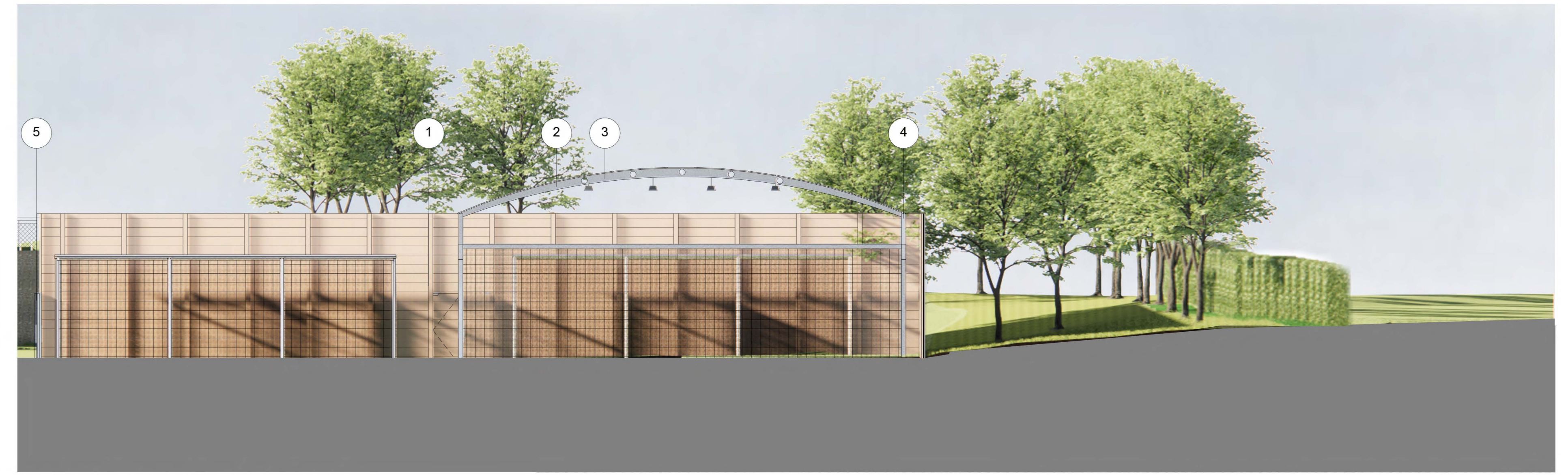
Practice Nets - North Elevation 1 : 100
