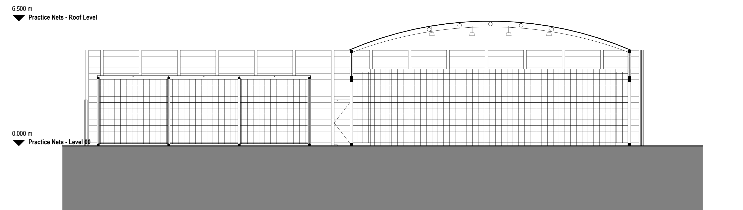
Practice Nets - Cross Section 1 : 100
