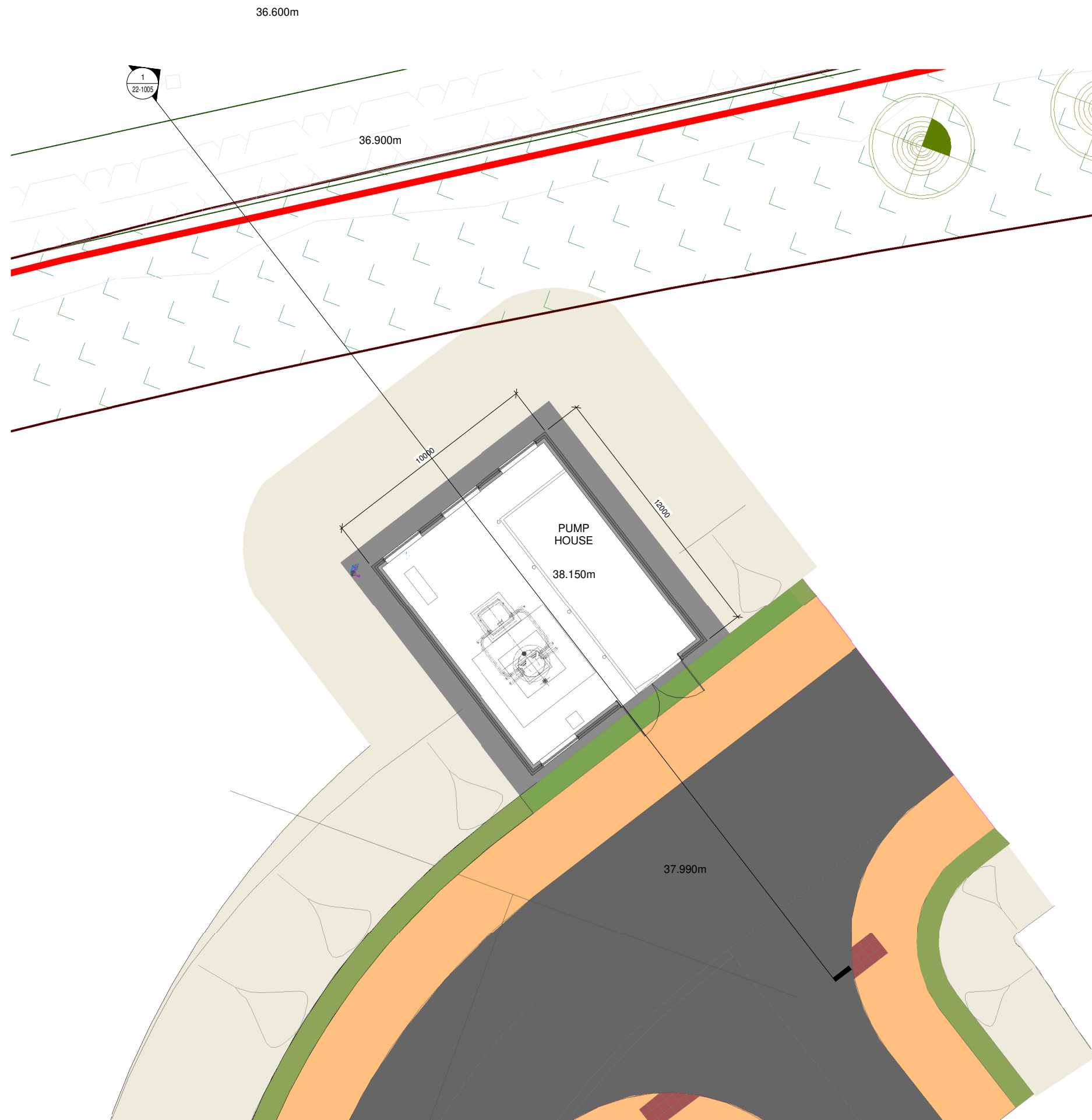
1 Proposed GA Pump House Plan 1 : 100
