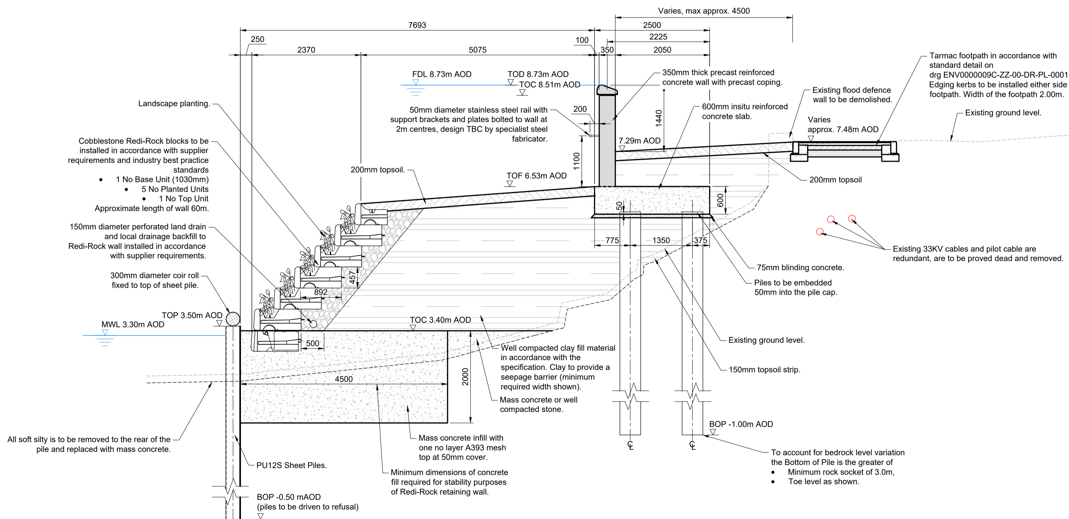
E-E Section E-E REF.1 SCALE 1:50
