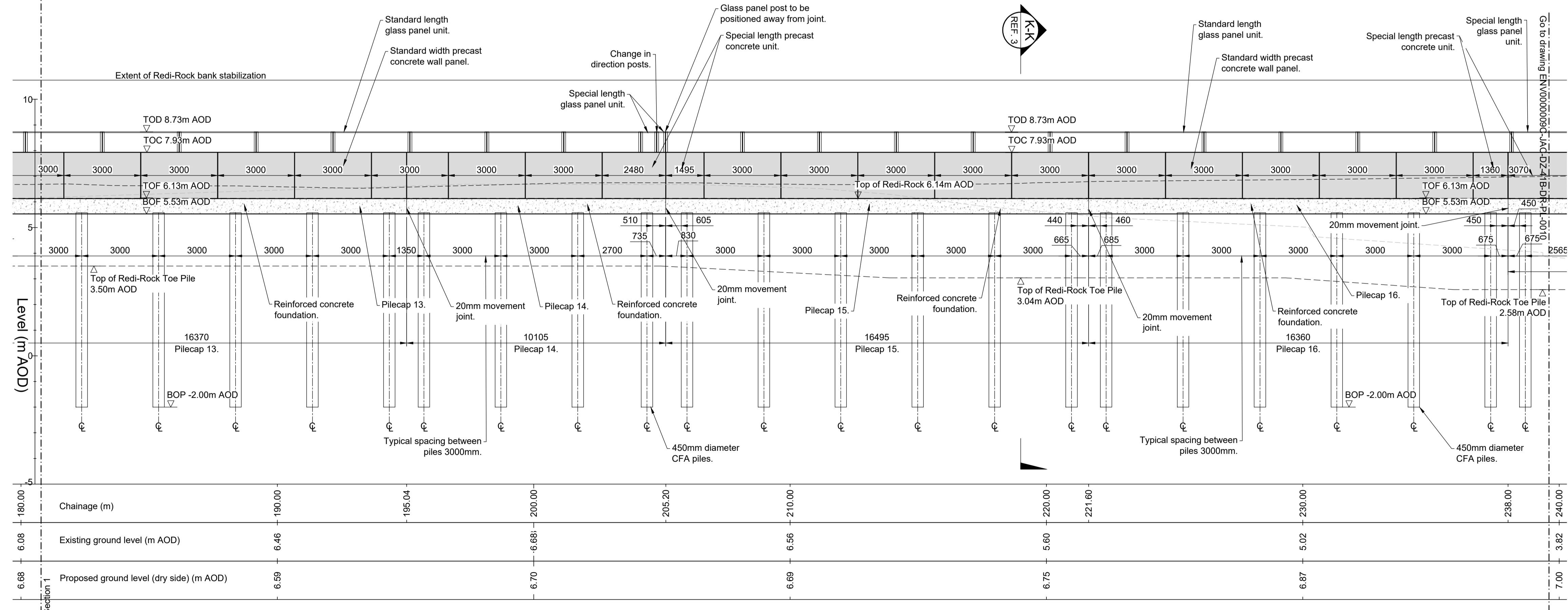
2 Longitudinal Section CH 180.00 to 240.00 SCALE 1:100
