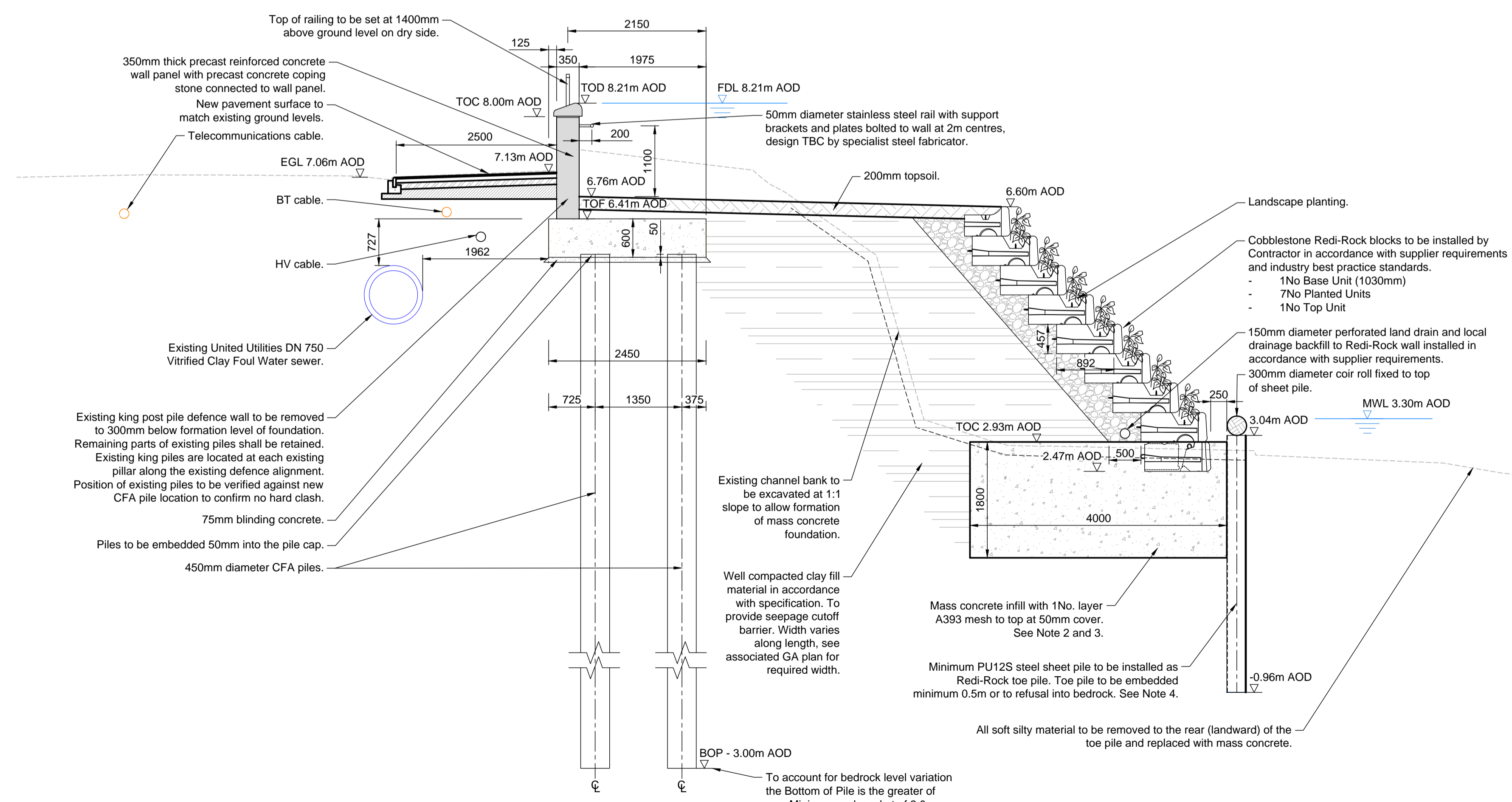
N-N Section N-N REF.2 SCALE 1:50
