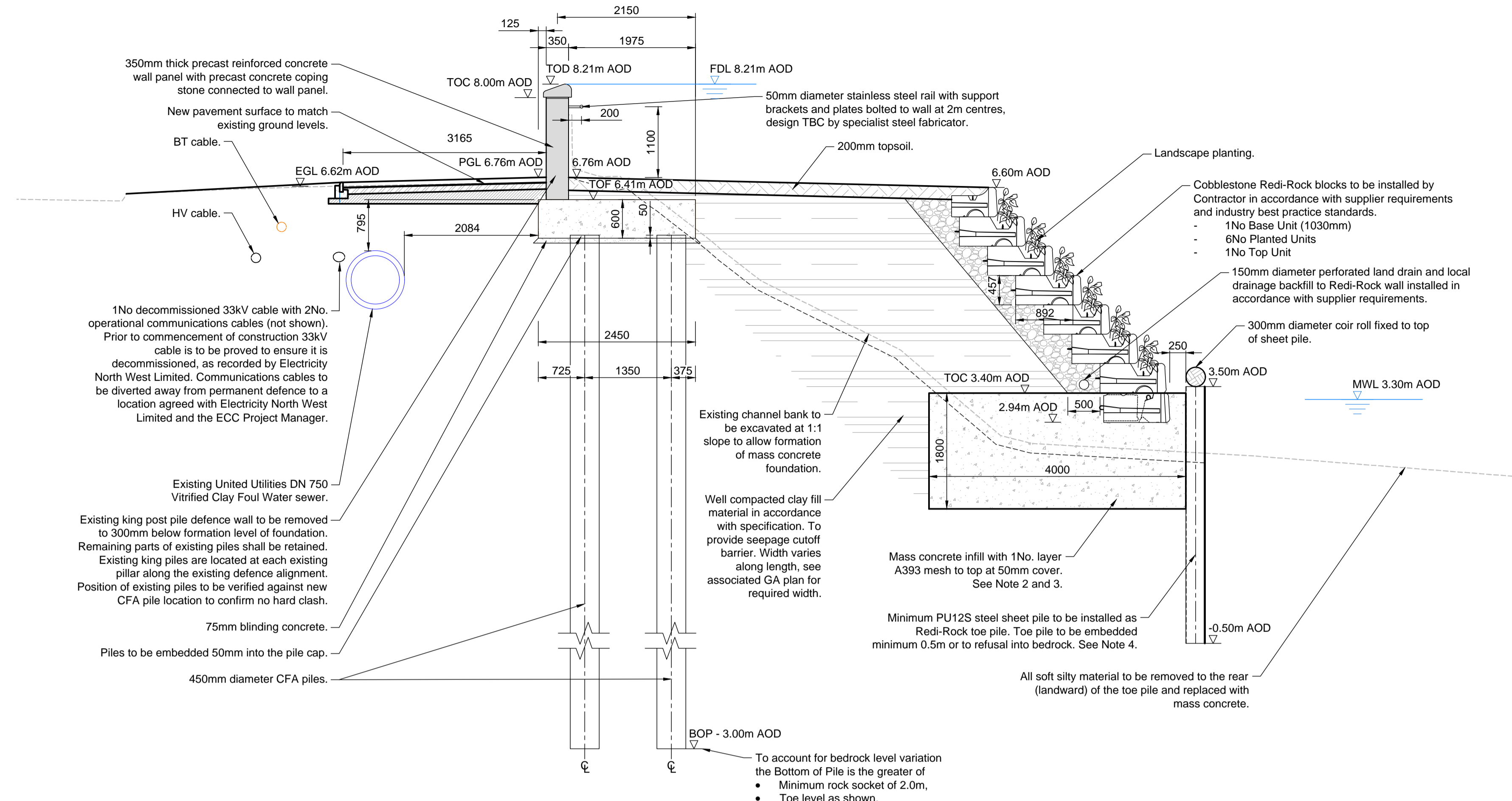
M-M Section M-M REF.2 SCALE 1:50
