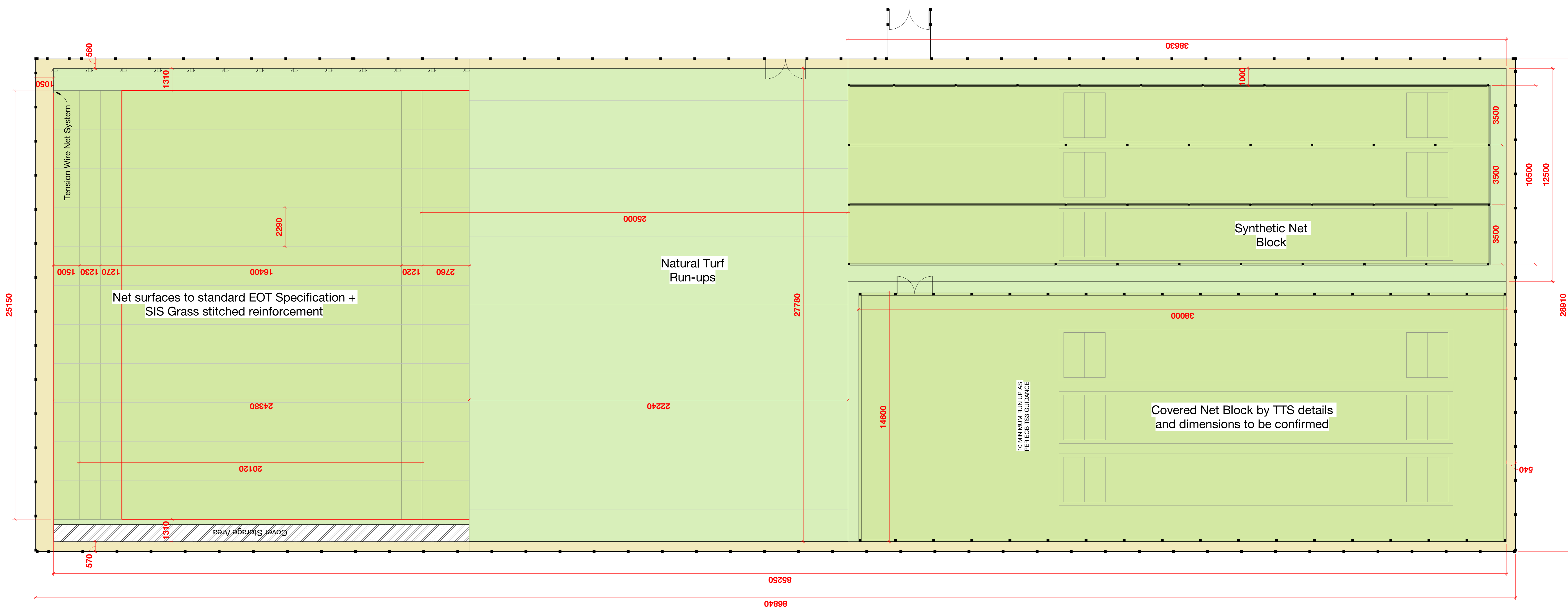
(0-) Practice Nets Floor Plan 1 : 100
