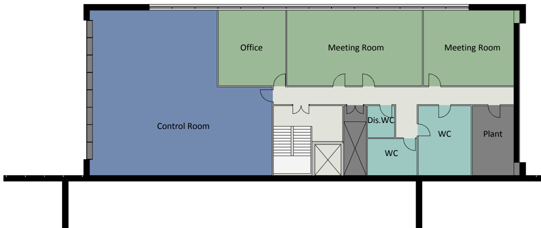
Office Plan - Level 03 1 : 200
