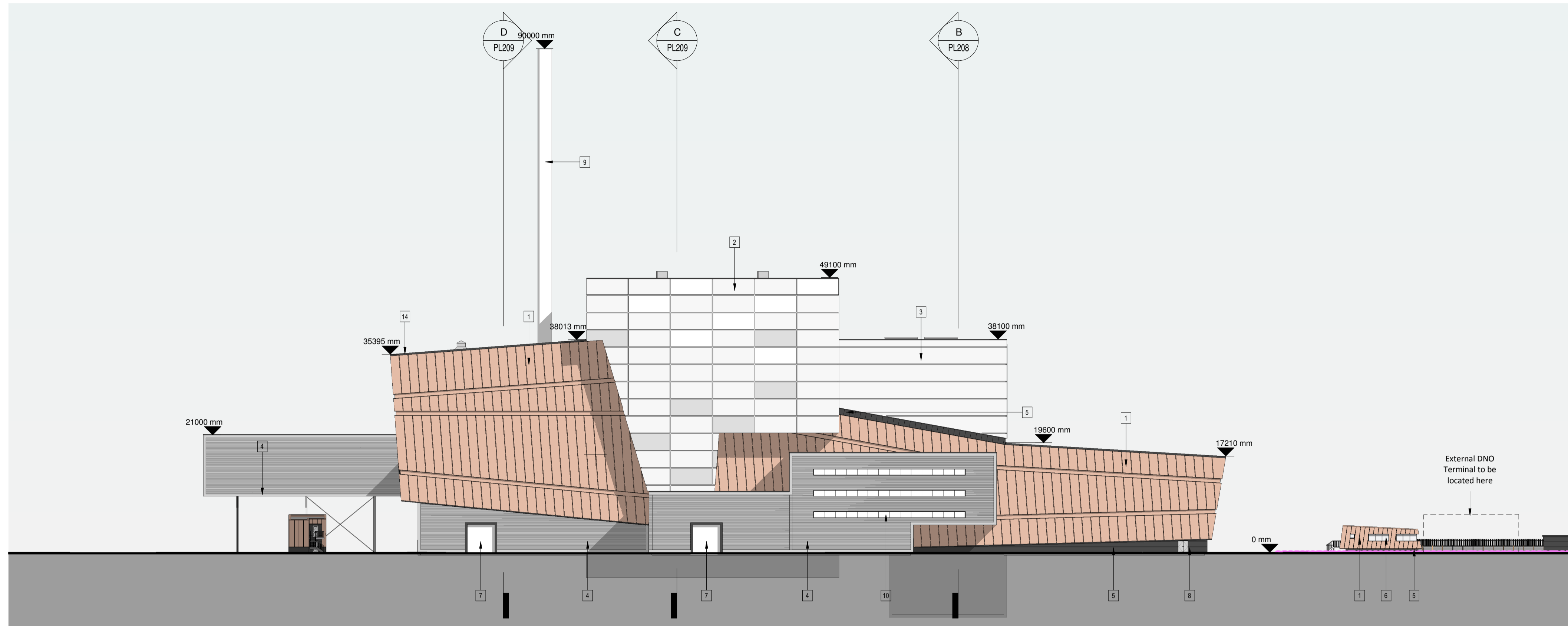
NORTH_PROPOSED 1 : 500
