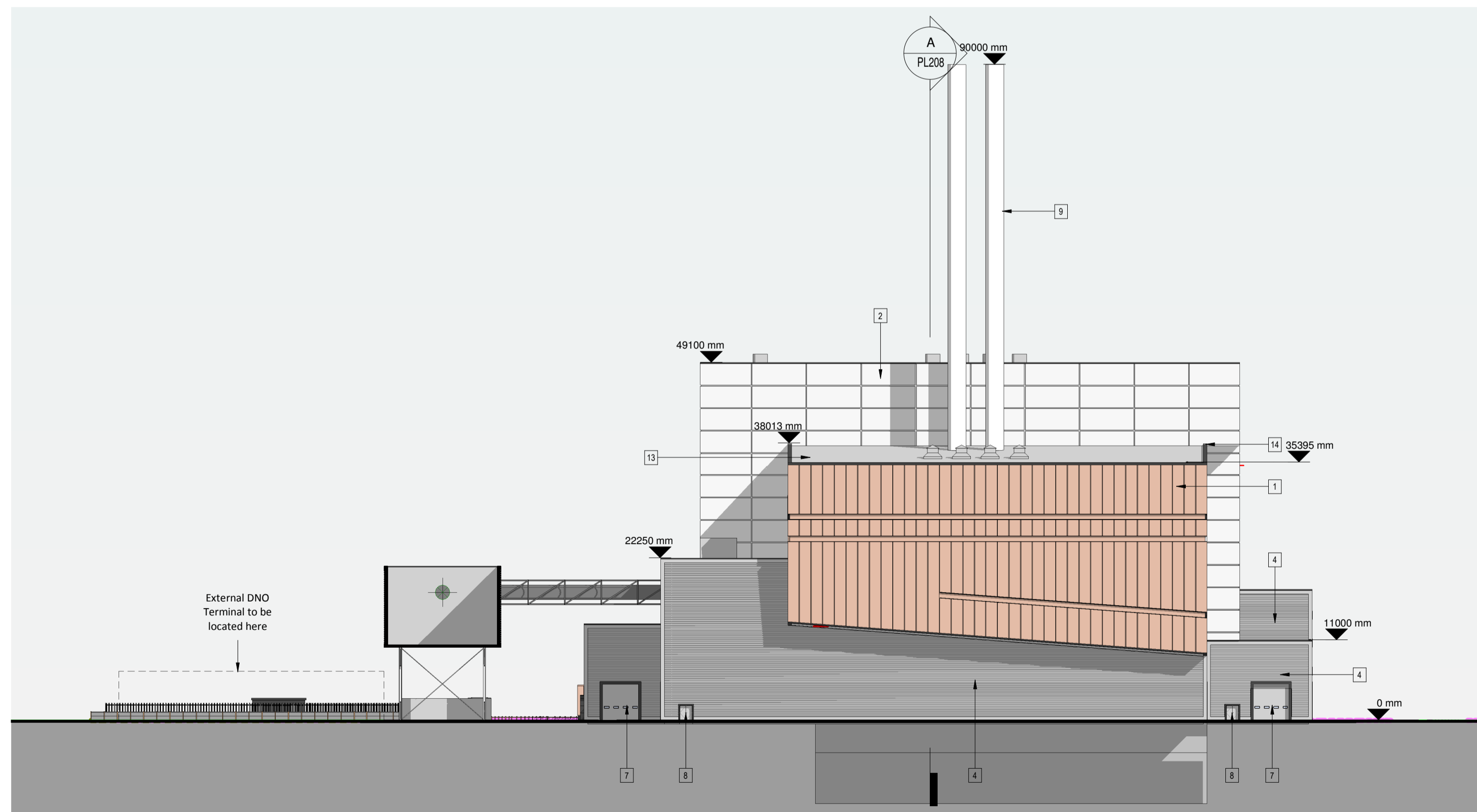
EAST_PROPOSED 1 : 500
